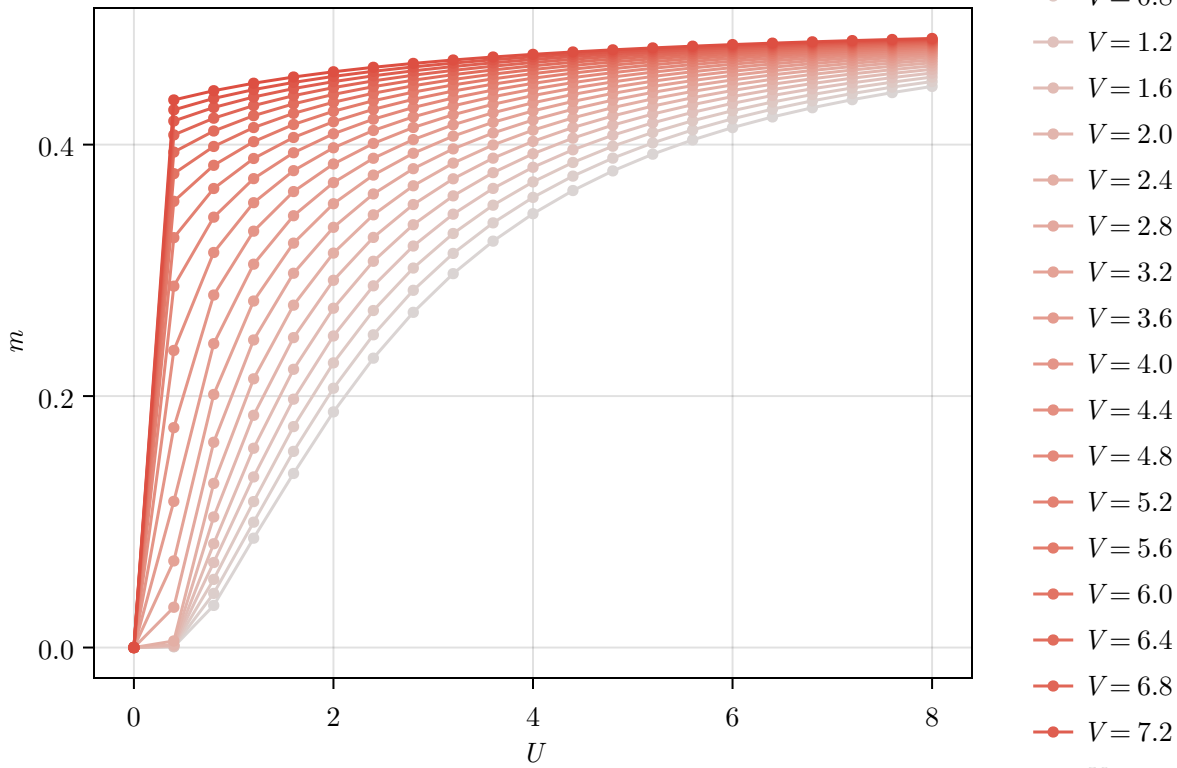
Magnetization ( t = 1.0 , L = 256 , \delta = 0.0 , \beta = 100.0 )
